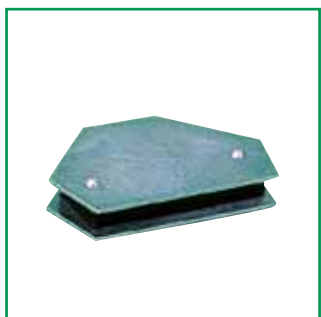
Mitre magnet Mitre magnet for 30°, 45°, 60°, 75° and 90°. Retaining power 1 x 300 N Article no. ....81080003
