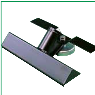
PM 300 mouthpiece * Rectangular extraction mouth- piece, 300 mm wide, with magnetic foot. For ø45 extraction hose. Article no. ....82031002
