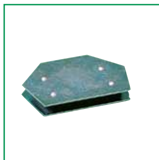
Mitre magnet Mitre magnet for 30°, 45°, 60°, 75° and 90°. Retaining power 1 x 450 N Article no. ....81080005
